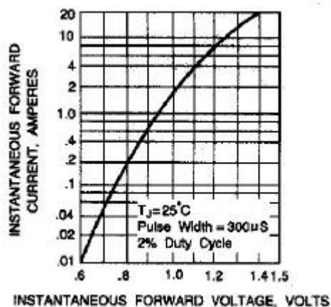
Fig. 2-TYPICAL FORWARD CHARACTERISTICS
