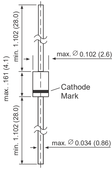
DO-204AL (DO-41 Glass)
