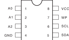
8-Pin TSSOP
