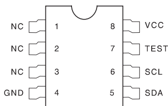
8-Pin SOIC
