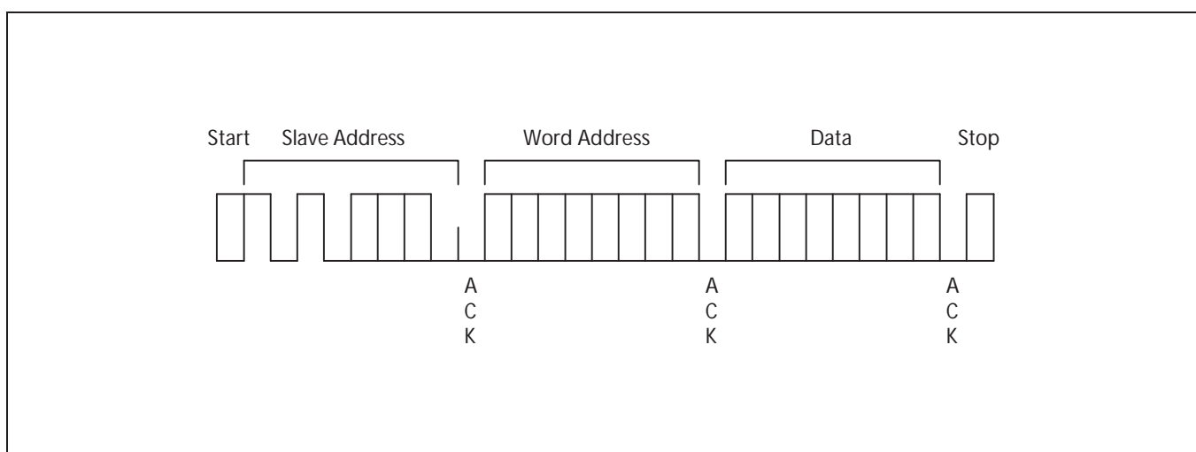
Figure 1-9. Byte Write Operation
