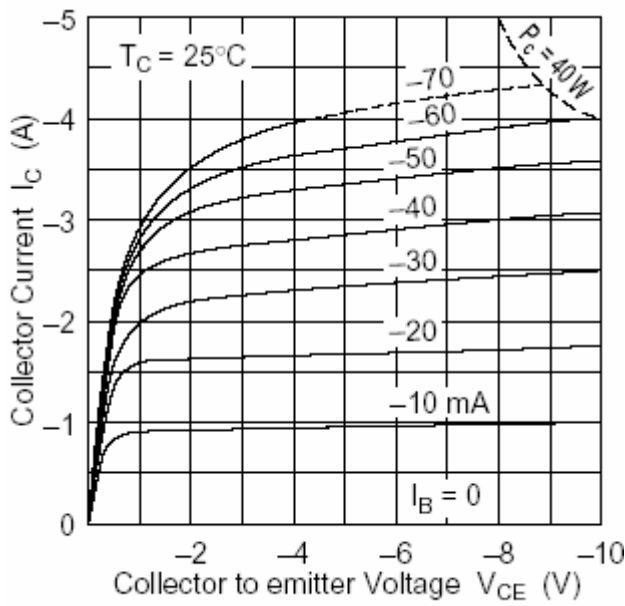
Fig.3 Static Characteristic
