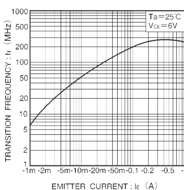
Fig.11 Gain bandwidth product vs. emitter current
