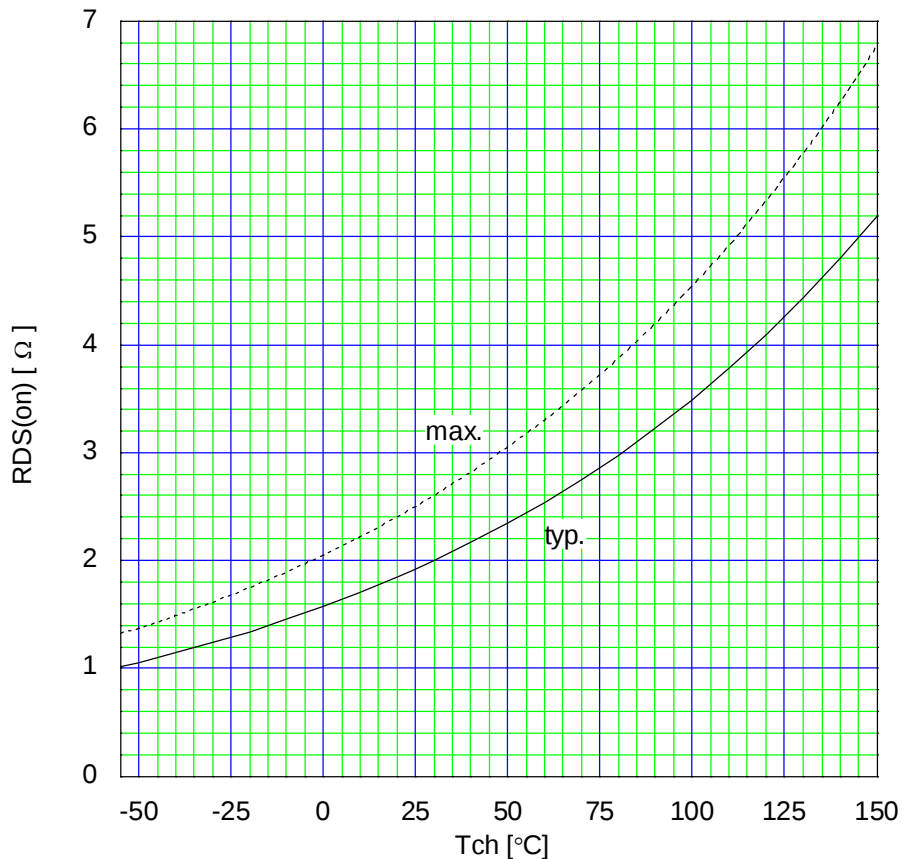
Drain-Source On-state Resistance R_{DS(on)}=f(T_{ch}):I_D=3\text{A}, V_{GS}=10\text{V}
