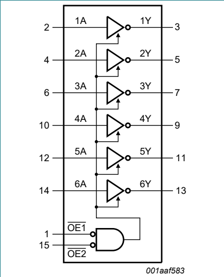
Fig. 1. Functional diagram
