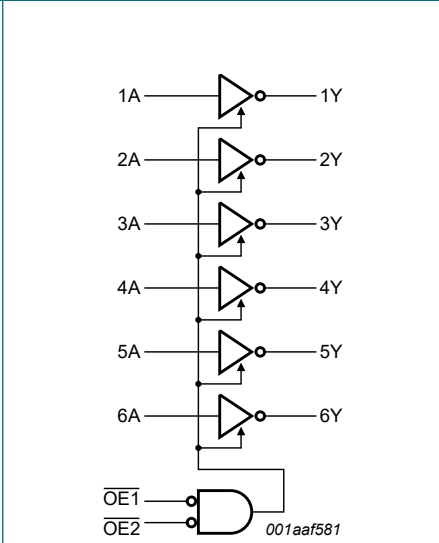
Fig. 2. Logic symbol
