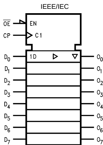
Figure 1. Logic Symbol
