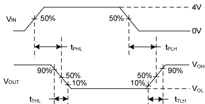
VOLTAGE WAVEFORMS
