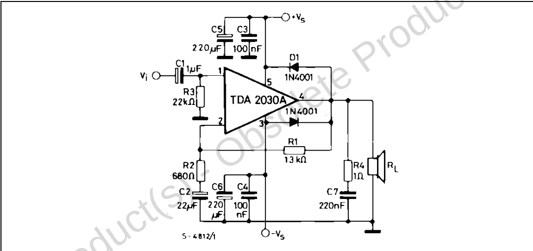
Figure 3. Test circuit
