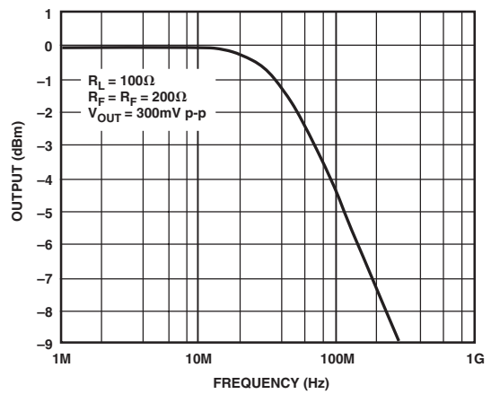
TPC 17. AD8047 Small Signal Frequency Response, G = -1
