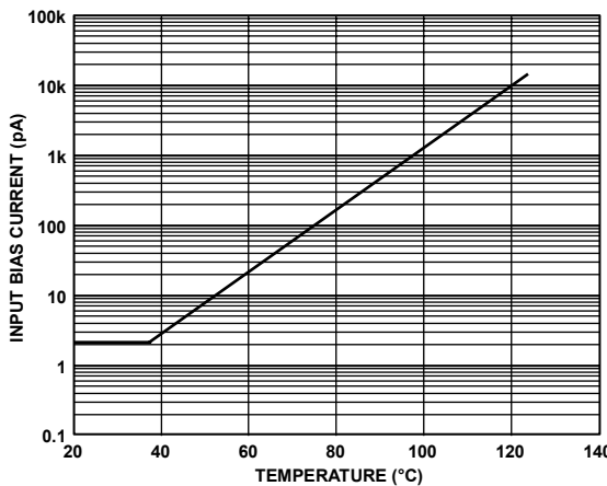
Figure 9. Input Bias Current vs. Temperature; V_S = 5\text{ V}, V_{CM} = 0
