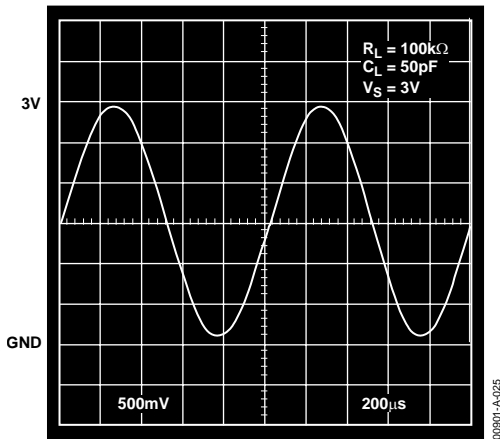
Figure 25. Output Swing, V_S = 3V , G = +1
