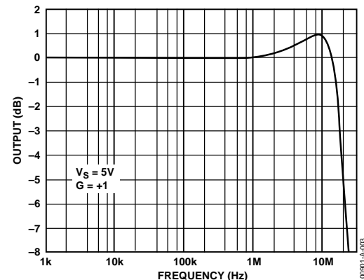
Figure 3. Small Signal Bandwidth, G = +1
