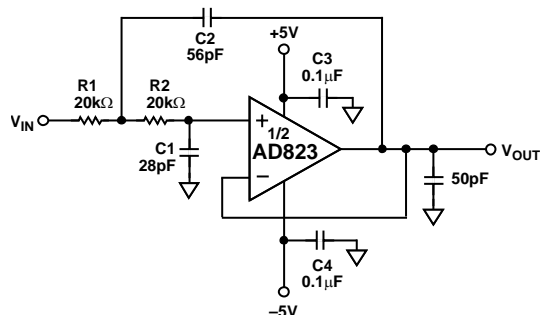
Figure 43. Second-Order Low-Pass Filter
