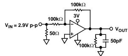
Figure 28. Output Swing, V_S = 3V , G = -1
