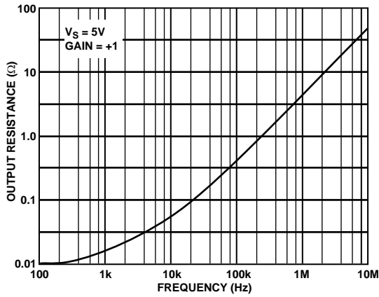
Figure 18. Output Resistance vs. Frequency, V_S = 5V , Gain = +1
