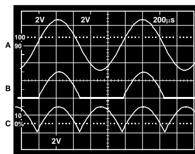
Figure 46. Single-Supply Half-Wave and Full-Wave Rectifier
