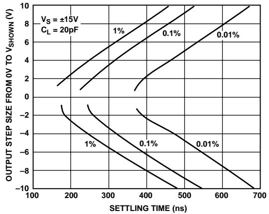
Figure 19. Inverter Settling Time vs. Output Step Size
