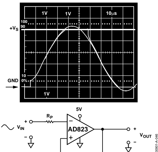
Figure 39. AD823 Input Response: V_{IN} = 0 to +V_S + 200\text{ mV} , V_{OUT} = 0 to +V_S , R_P = 49.9\text{ k}\Omega
