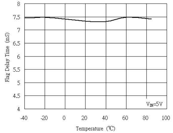
Fig. 8 Flag Delay Time vs. Temperature
