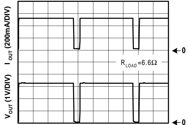
Overtemperature Shutdown
