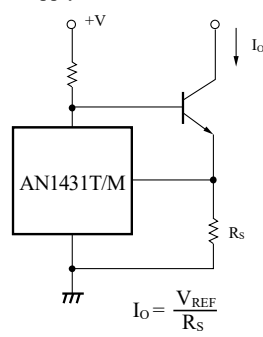
2. Constant Current Power Supply
