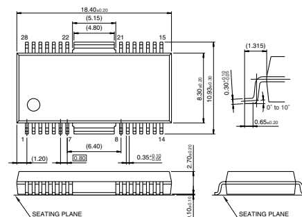
HSOP042-P-0400
