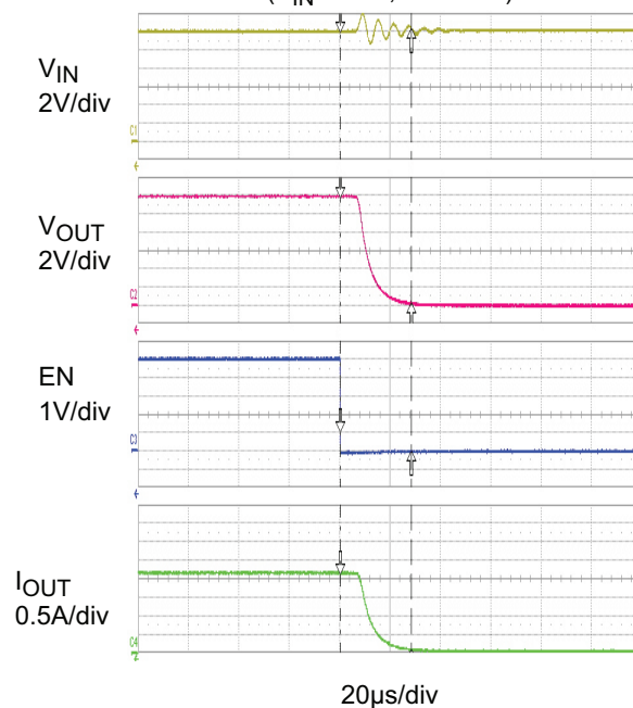
Turn-Off ( V_{IN} = 12V , R = 5.6\Omega )
