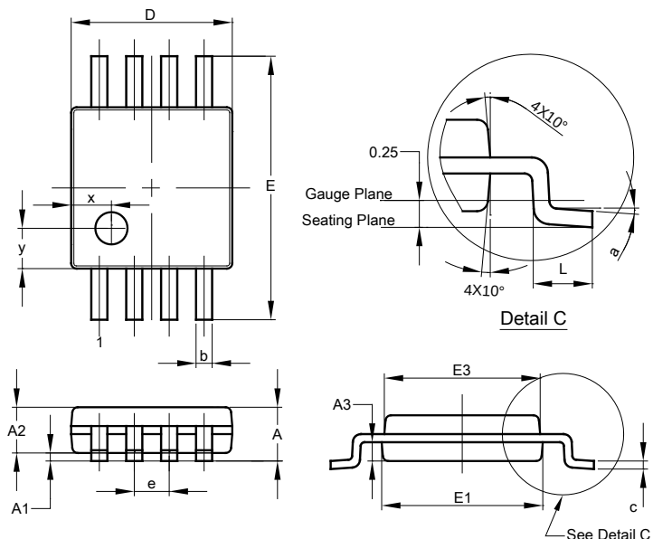
MSOP-8
