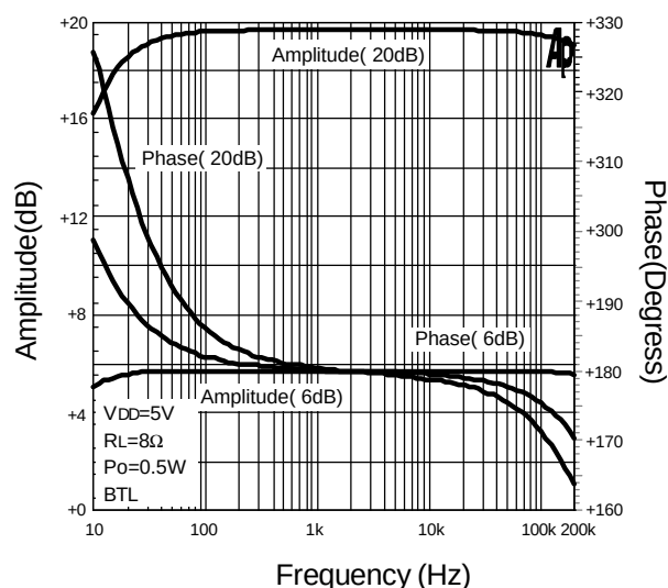
Frequency Response
