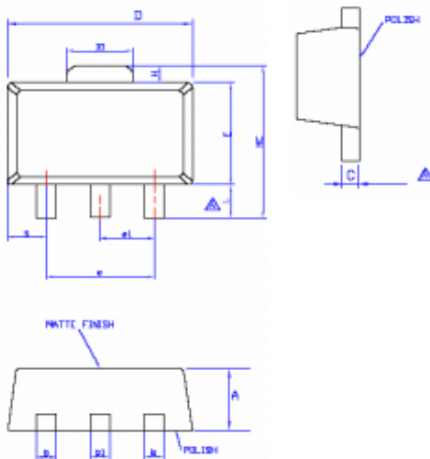
SOT-89 Package (Unit: mm)
