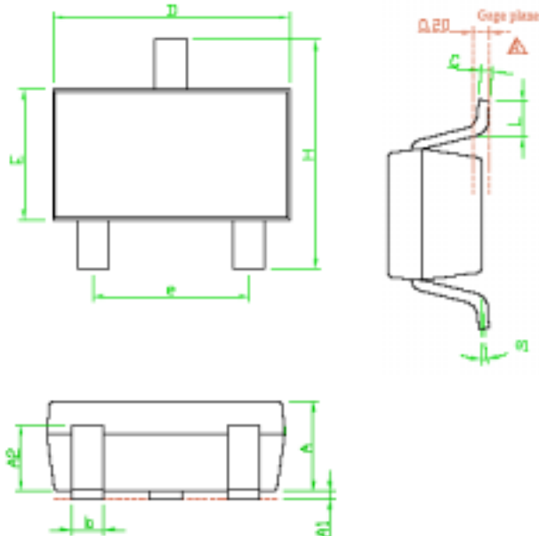
SOT-23 Package (Unit: mm)
