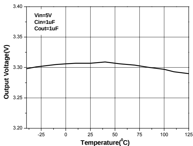
Figure 13. Temperature Stability
