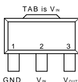
SOT-89 (Top View) APL5508
