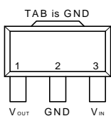
SOT-89 (Top View) APL5509
