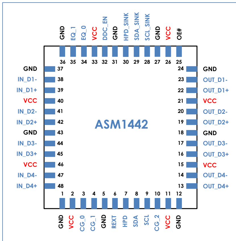
Figure 4: ASM1442 pinout
