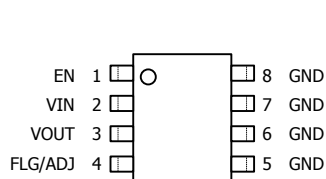
SOP-8
