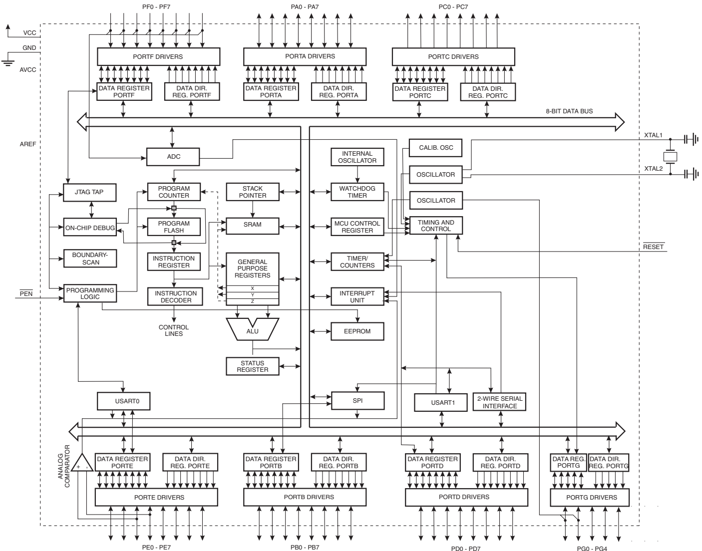
Figure 2. Block Diagram
