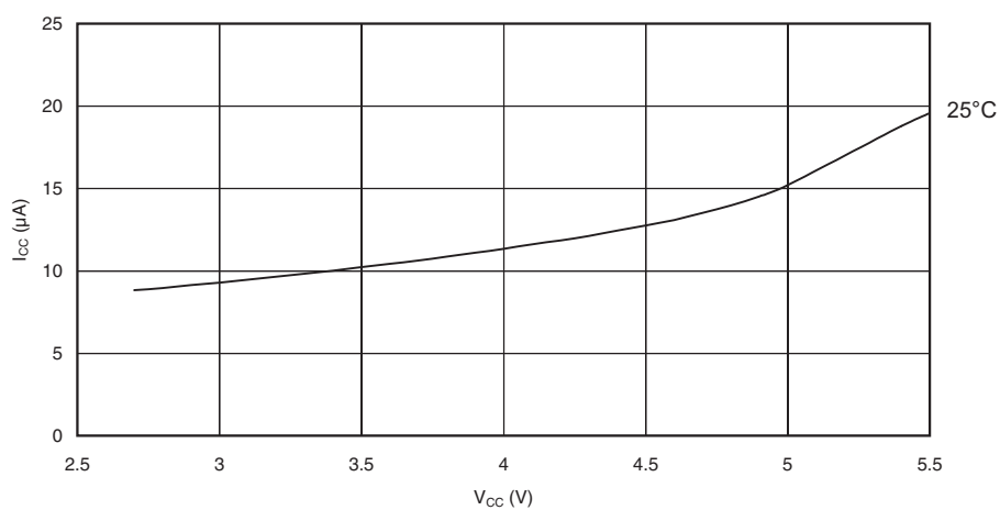
Figure 134. Power-save Supply Current vs. V_{CC} (Watchdog Timer Disabled)
