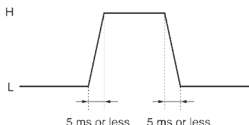
Fig.17 Control signal
