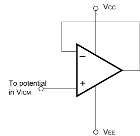
Fig.11 Unused circuit connections
