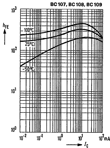
DC current gain h_{FE} = f(I_C) ; V_{CE} = 5\text{ V} ; T_{amb} = parameter (common emitter configuration)
