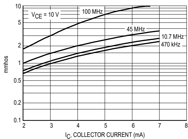
Figure 7. g11e (gie)
