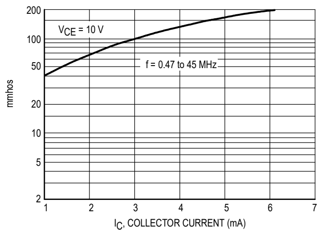
Figure 8. g21e (Yfe)
