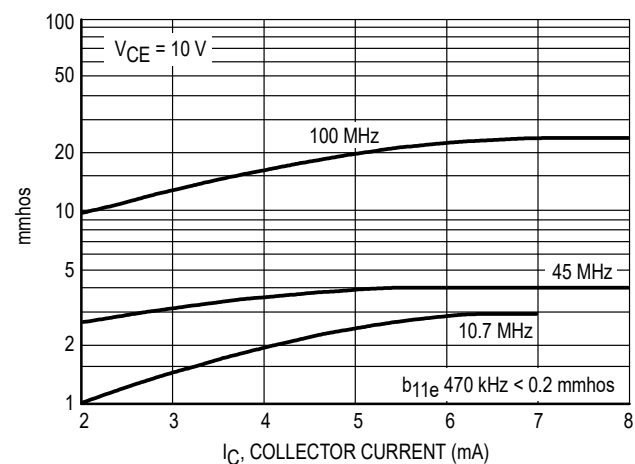
Figure 4. b11e
