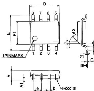
Fig.-4 SO8 narrow Package Outline
