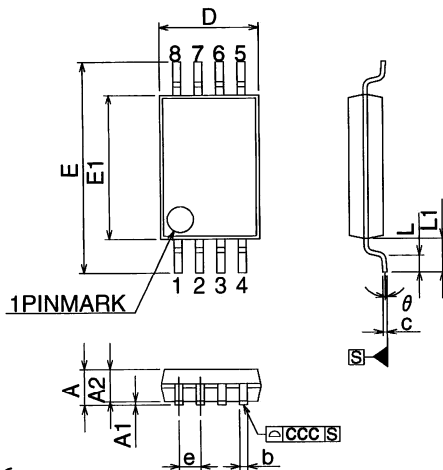
Fig.-4 SO8 narrow Package Outline
