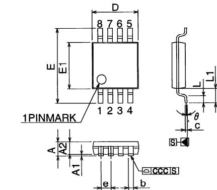
Fig.-5 TSSOP Package Outline
