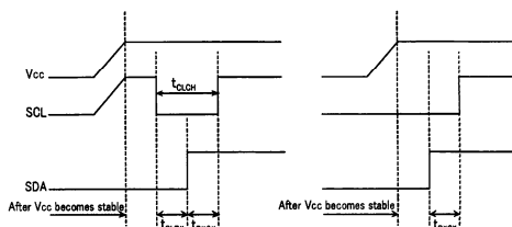
Fig.-3(a) SCL='H' and SDA='L'
