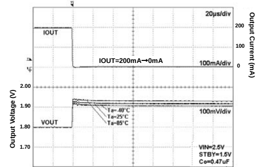
Fig 19. Load Response
