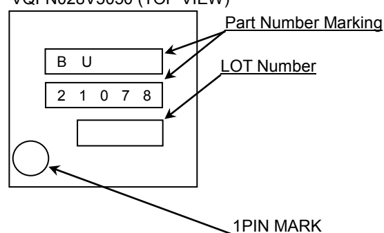
VQFN028V5050 (TOP VIEW)
