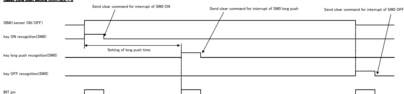
Figure 23. Interrupt of simple switch (1)
