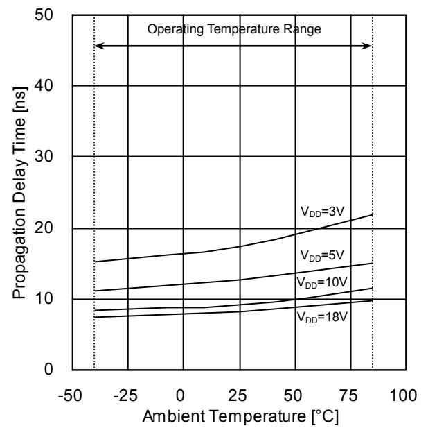
Figure 12. Propagation Delay Time t_{PLH} (IN→OUT) vs Ambient Temperature
