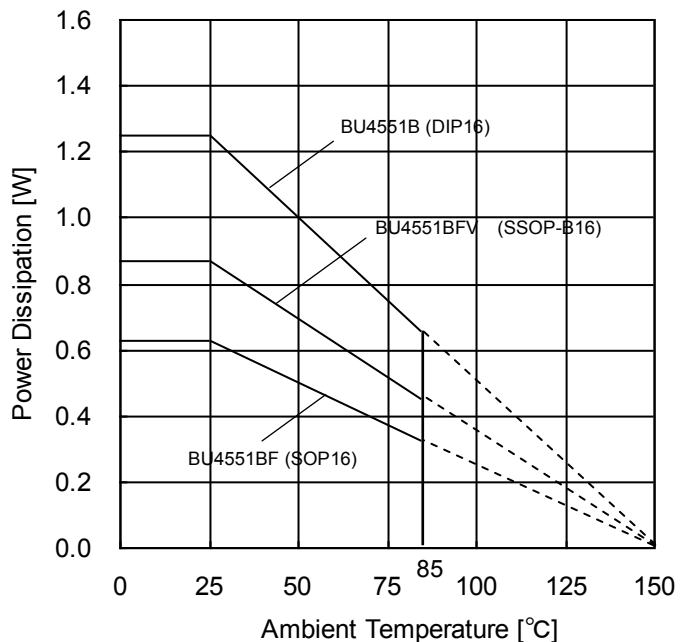
Figure 18. Derating Curve
