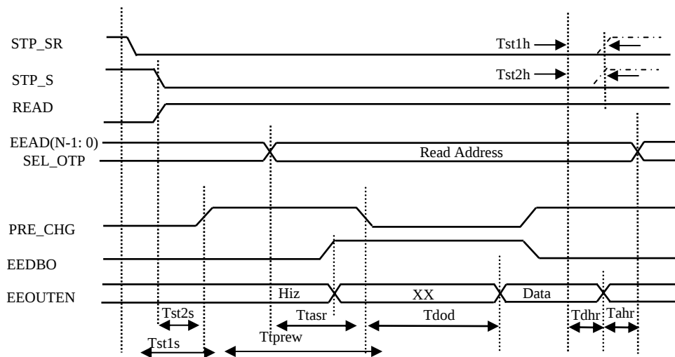
Figure4-1. Read mode timing
