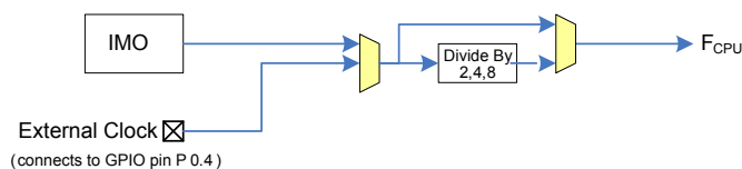
Figure 3. PSoC 4000 MCU Clocking Architecture
