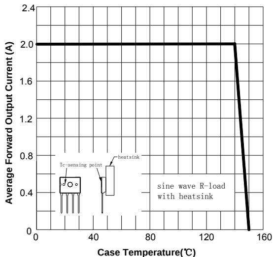
FIG1:Io-Tc Curve
