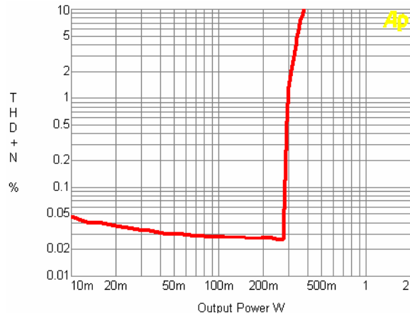
THD + Noise vs Output Power
