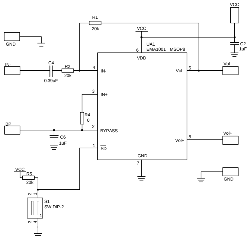
FIGURE 3. REFERENCE DESIGN
