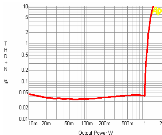
THD + Noise vs Output Power @ V_{DD} = 5.0V , R_L = 8\Omega , 1kHz , A_v = 2
