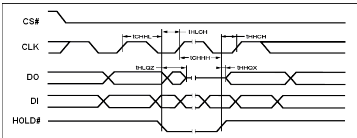
Figure 25. Hold Timing
