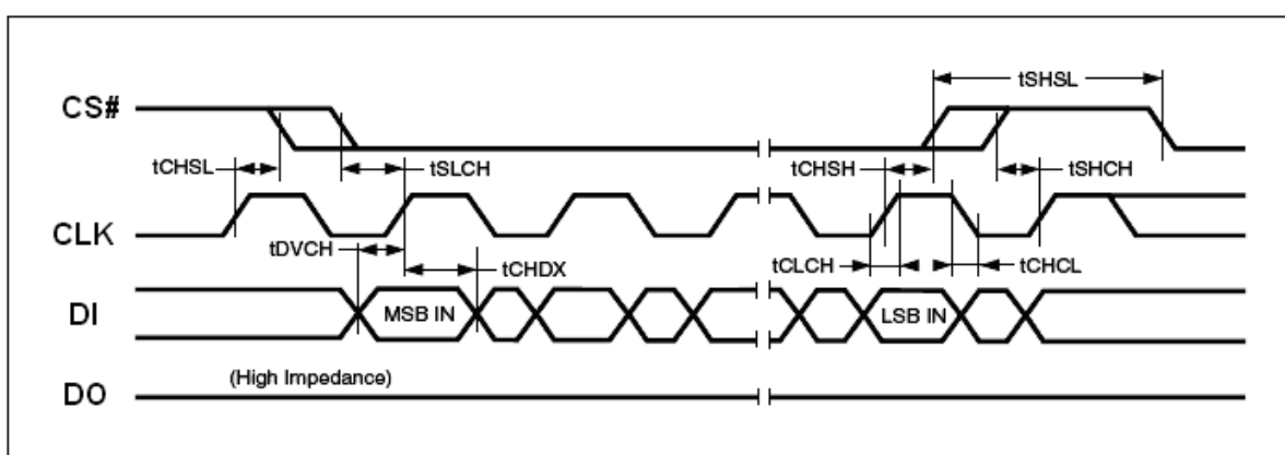
Figure 24. Input Timing
