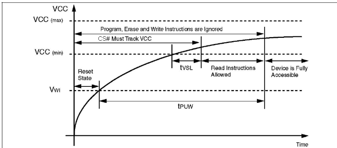
Figure 27. Power-up Timing
