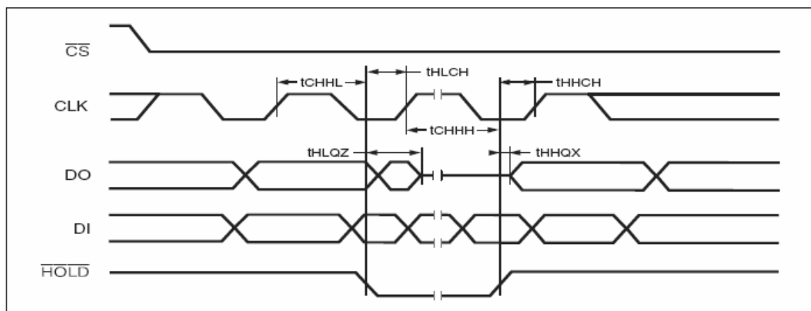
Figure 26. Hold Timing
