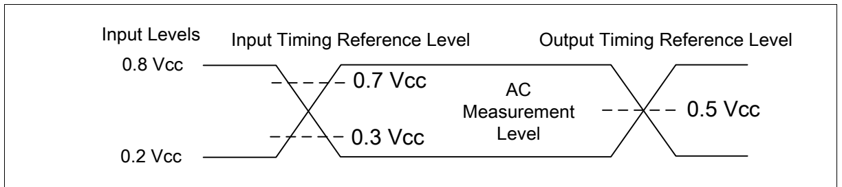
Figure 82 AC Measurement I/O Waveform
