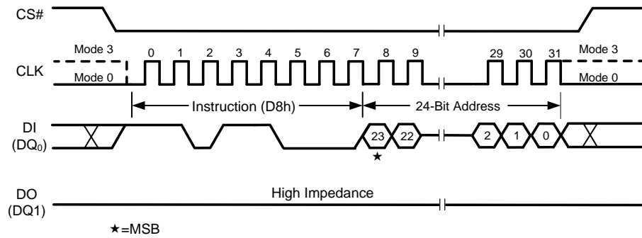
Figure 43 64KB Block Erase Instruction (SPI Mode)
