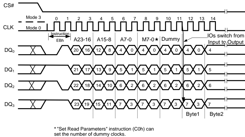
Figure 30 Fast Read Quad I/O Instruction (Initial instruction or previous M5-4#10, QPI Mode)
