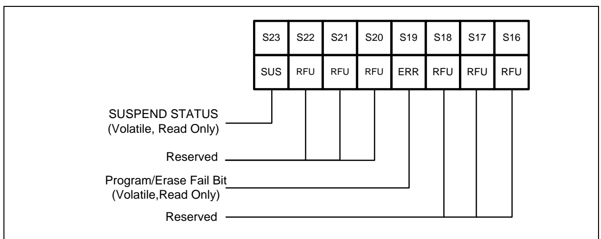
Figure 10 Status Register-3
