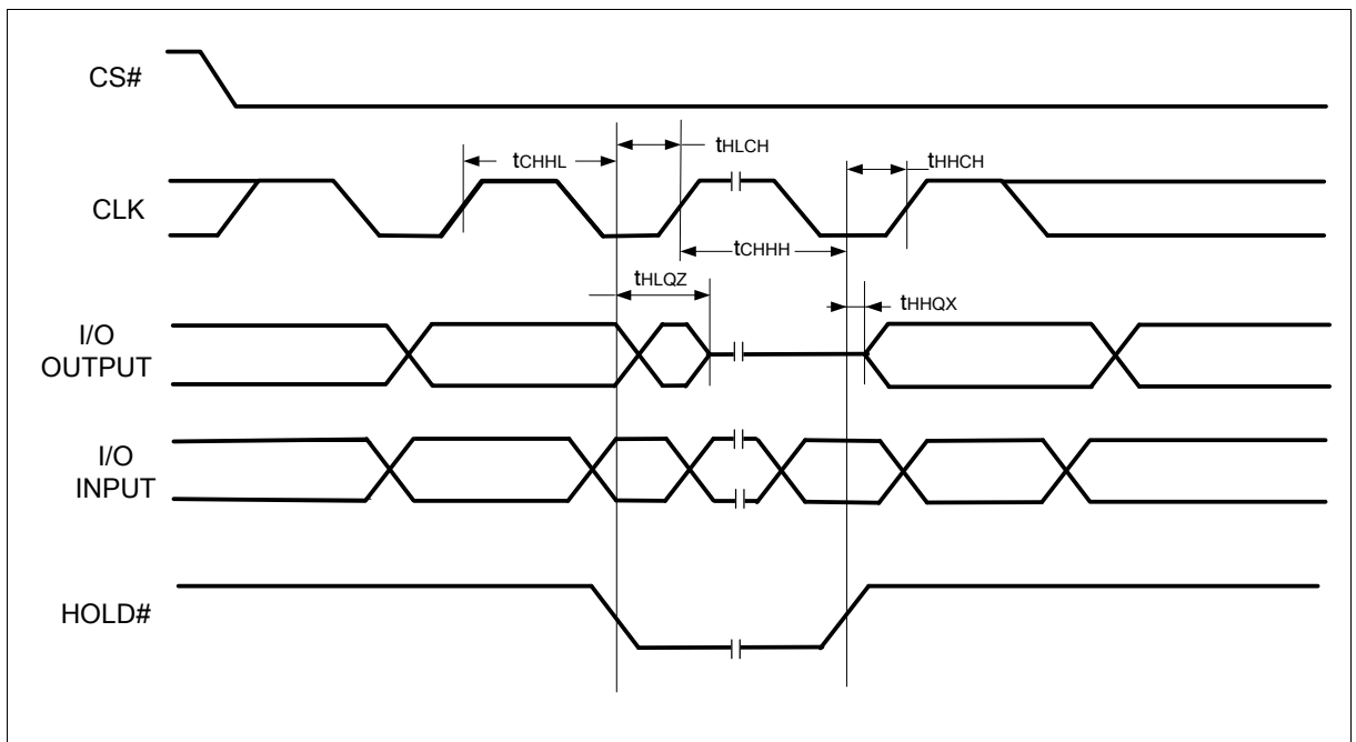
Figure 85 Hold Timing
