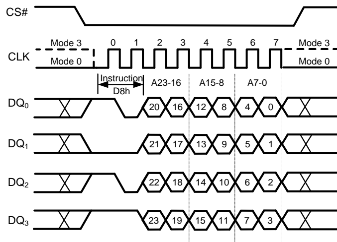
Figure 44 64KB Block Erase Instruction (QPI Mode)
