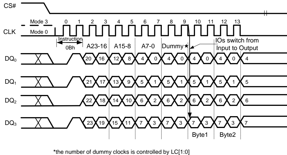
Figure 23 Fast Read Instruction (QPI Mode)
