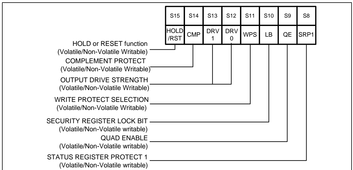
Figure 9 Status Register-2
