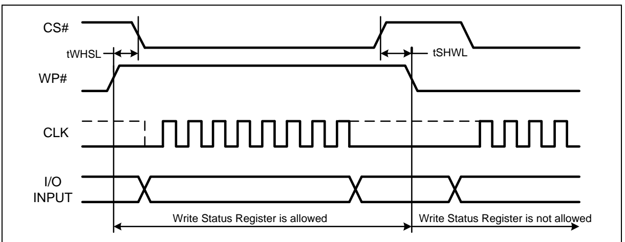
Figure 86 WP# Timing
