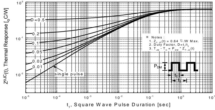
Figure 11-1. Transient Thermal Response Curve for FQP13N50C
