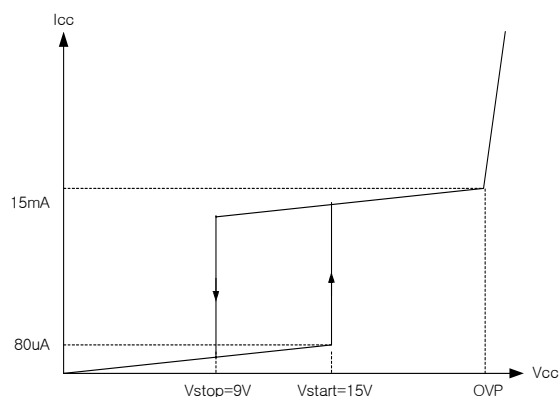
Figure 1. Strat up with hysteresis
