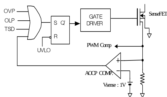
Figure 4. AOCP block
