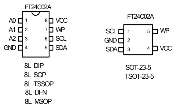
Figure 1: Package types
