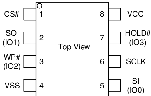
8 - LEAD VSOP/SOP
