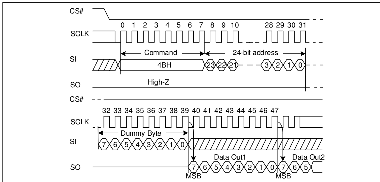
Figure 28. Read Unique ID Sequence Diagram
