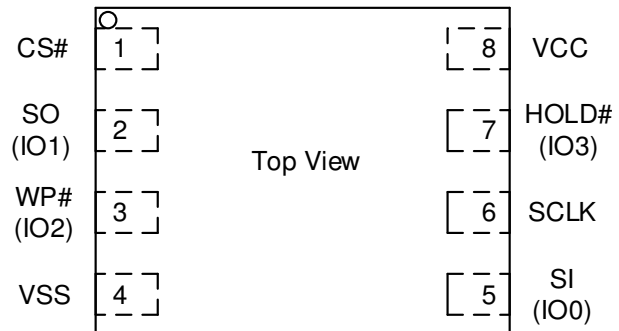
8 - LEAD WSON/USON
