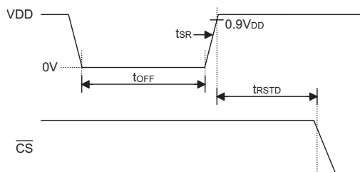
Figure 4 Power-on Reset Timing
